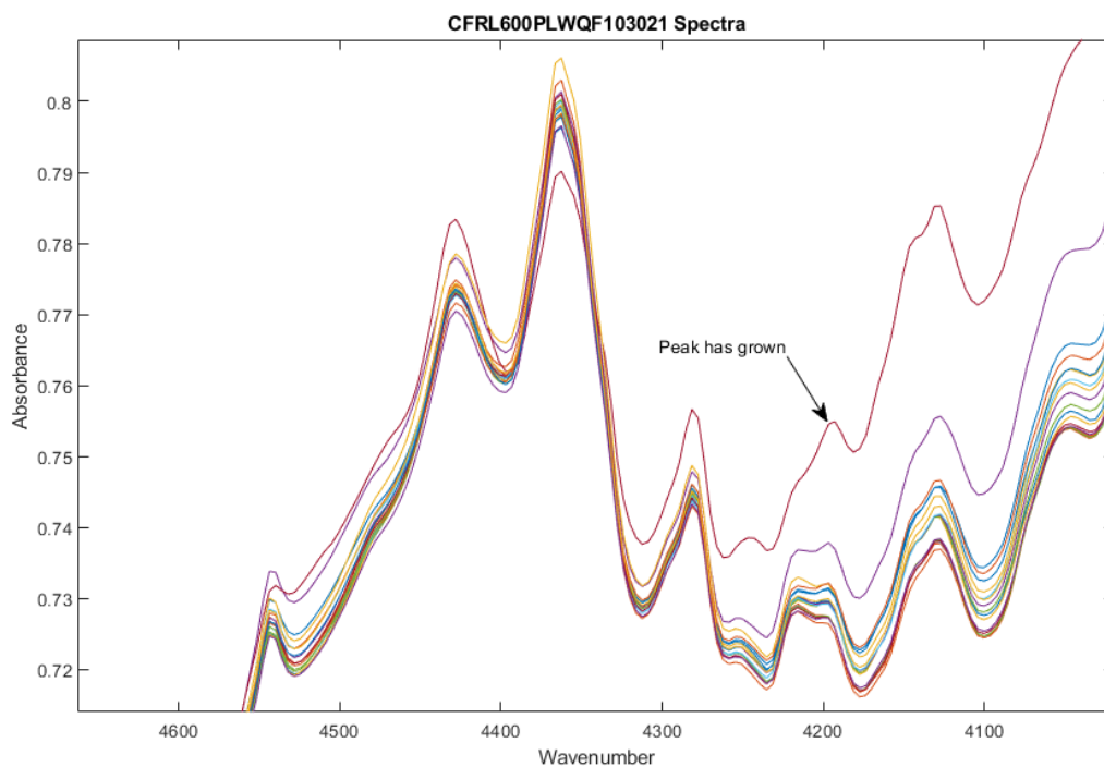
Figure 2. Zoom-in on spectra of 18 vials of Ceftaroline Fosamil from Lot0013E06 after multiplicative scatter correction. Some peaks have grown in vial 7 (shown in red), most notably at 4190\text{ cm}^{-1} .
